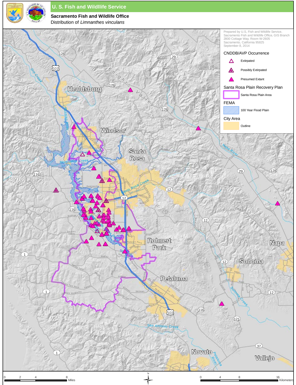
Figure 7. Distribution of Limnanthes vincularis (Sebastopol meadowfoam)
