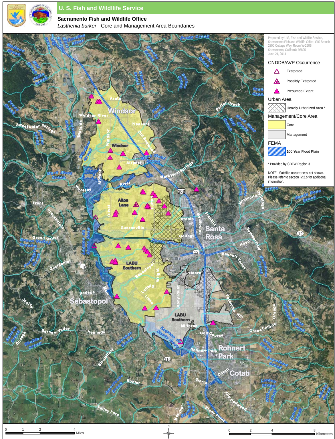
Figure 11. Lasthenia burkei Core and Management Area Boundaries on the Santa Rosa Plain
