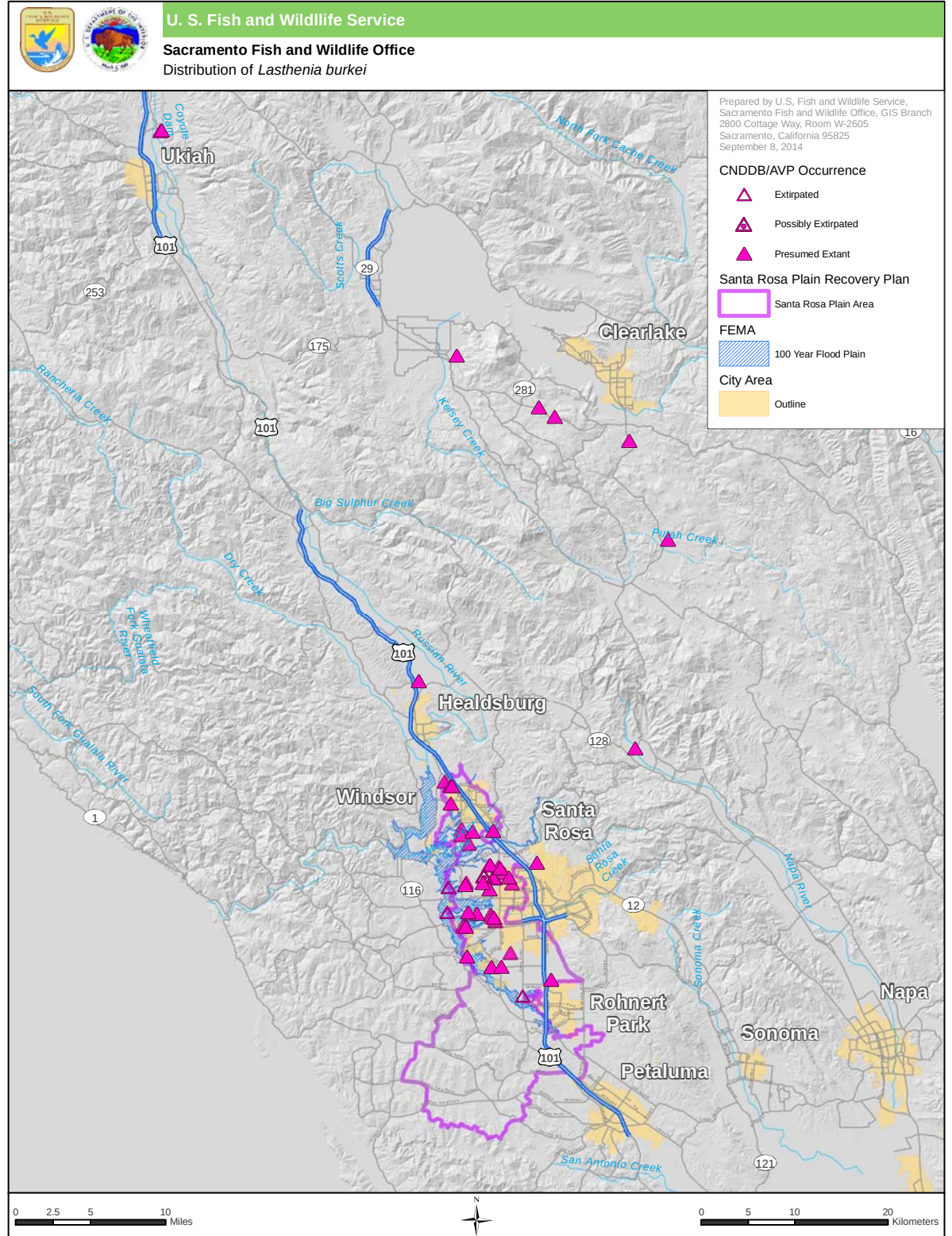
Figure 5. Distribution of Lasthenia burkei (Burke's goldfields)
