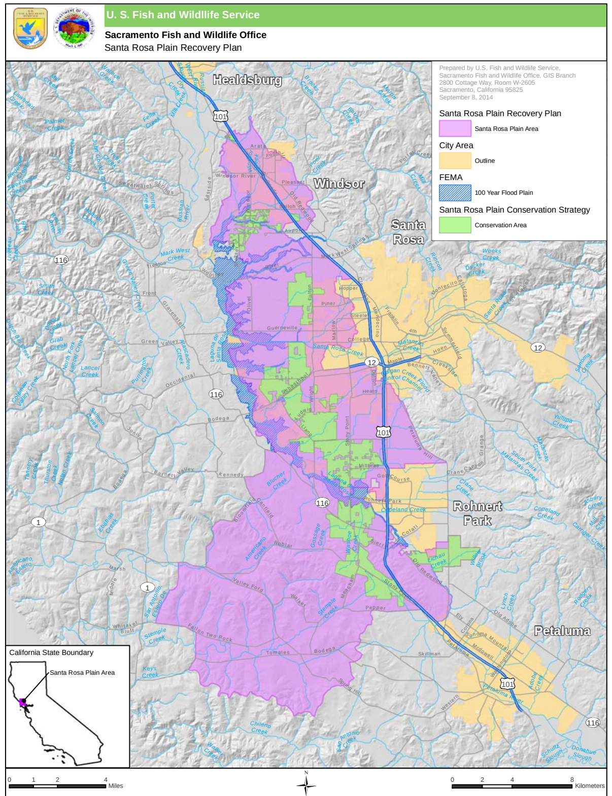
Figure 1. Santa Rosa Plain Portion of Recovery Planning Area
