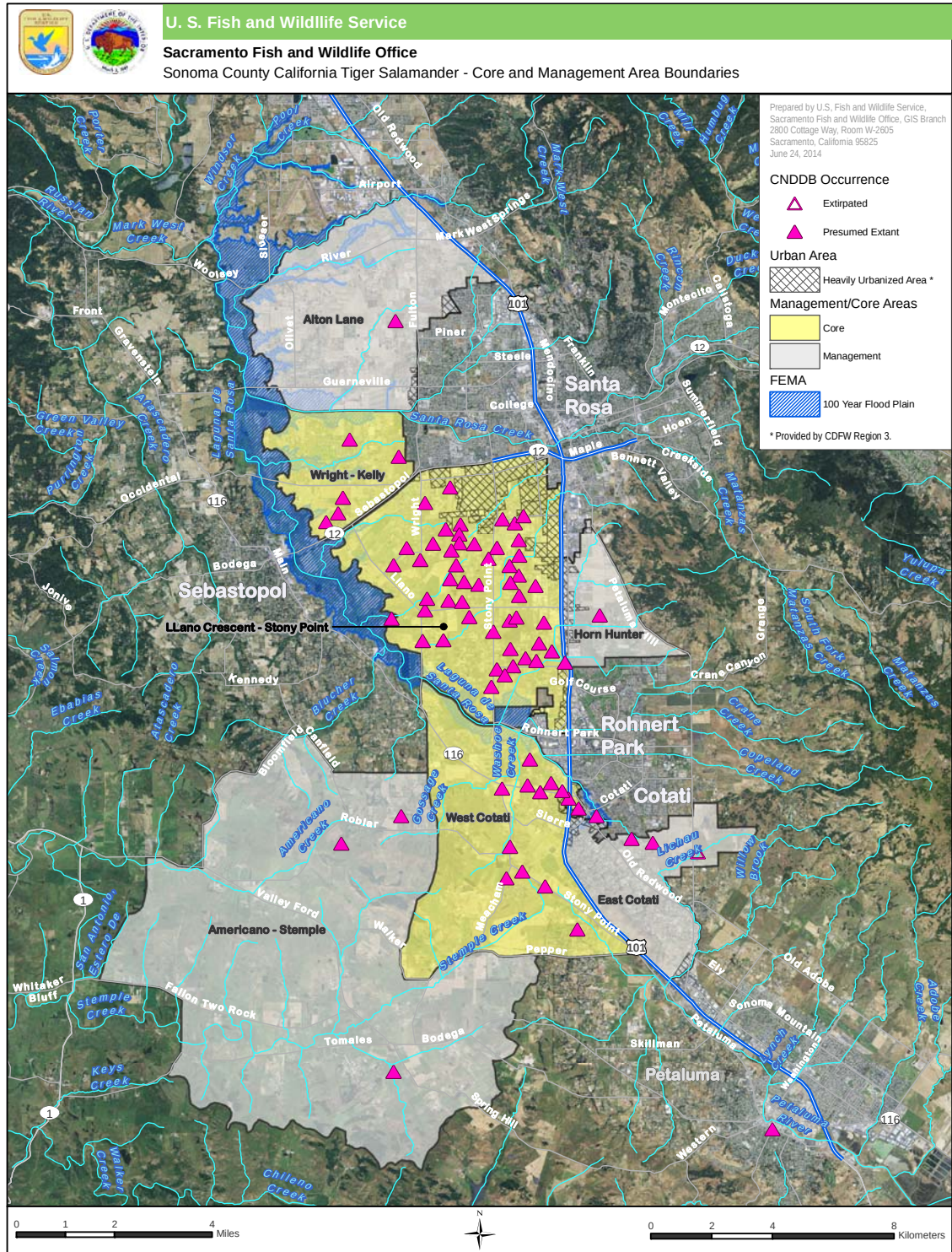
Figure 13. Sonoma County California Tiger Salamander Core and Management Area Boundaries on the Santa Rosa Plain
