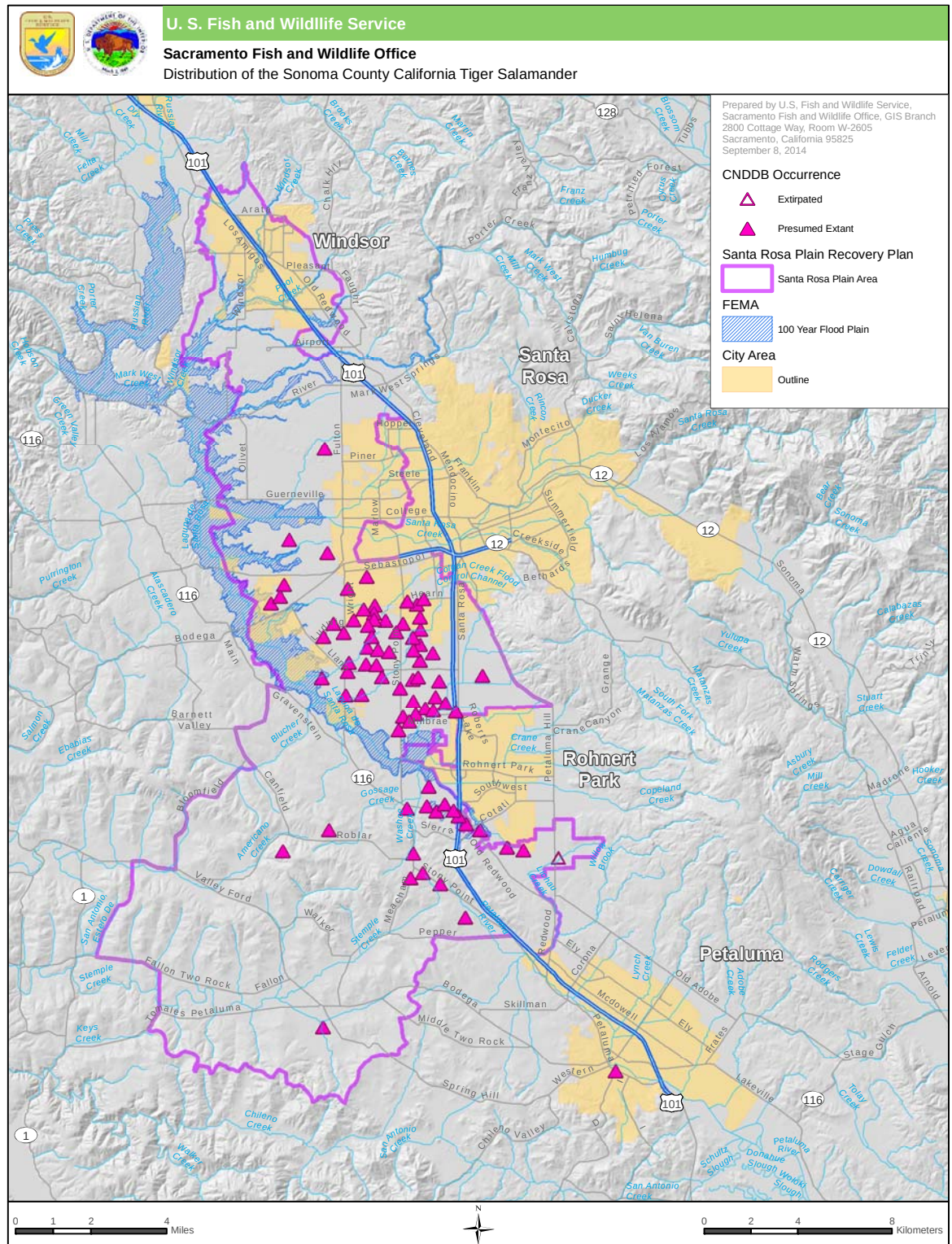
Figure 9. Distribution of the Sonoma County California Tiger Salamander
