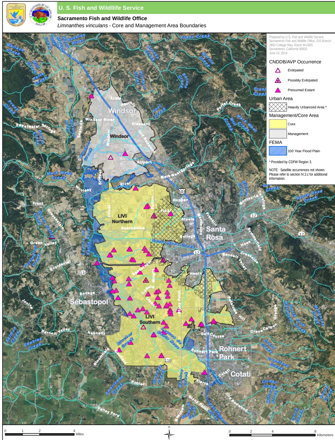
Figure 12. Limnanthes vincularis Core and Management Area Boundaries on the Santa Rosa Plain
