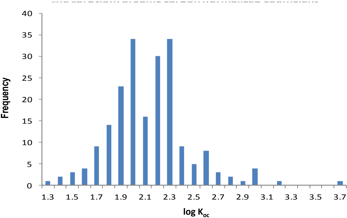
FIGURE 3-1 Organic-carbon normalized sorption coefficients, K_{oc} , values for atrazine plotted on a logarithmic scale. Source: Gerstl 1990. Reprinted with permission; copyright 1990, Journal of Contaminant Hydrology .
